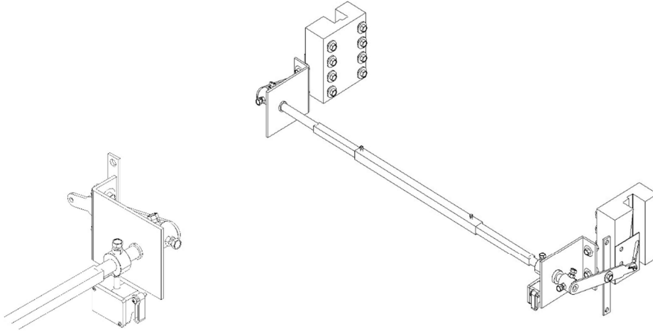
Safety gear synchronisation bar
